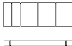
Cama | Colchão 150 x 195 Bed | Mattress 150 x 195 A 110 x L 162 x P 204
