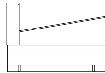
Cama | Colchão 150 x 195 Bed | Mattress 150 x 195 A 110 x L 162 x P 204
