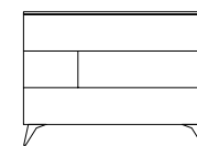
Cómoda c/ 3 gavetas Chest of drawers with 3 drawers A 91 x L 110 x P 45
