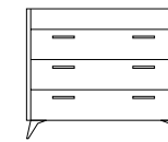
Cómoda c/ 4 gavetas Chest of drawers with 4 drawers A 94 x L 110 x P 45
